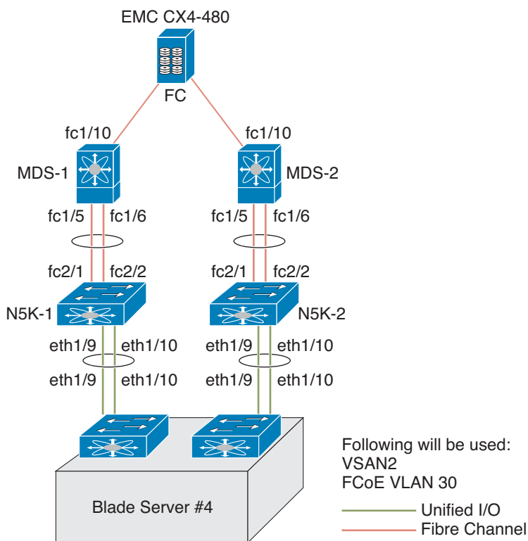
Figure D-1 Nexus 4000 FCoE Lab Topology
