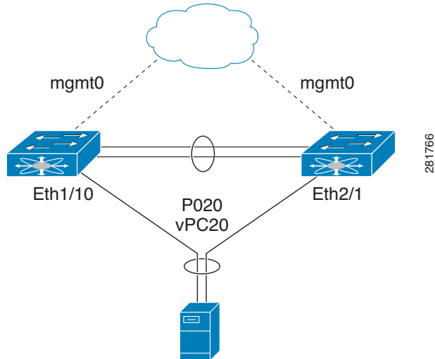
Figure 4-4 Switch vPC Topology
